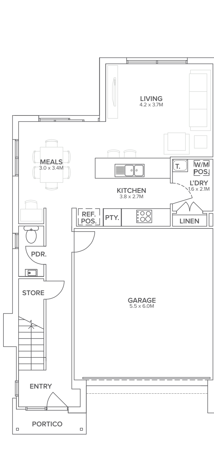
GROUND FLOOR
