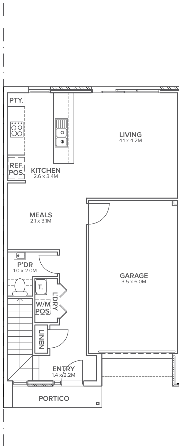
GROUND FLOOR
