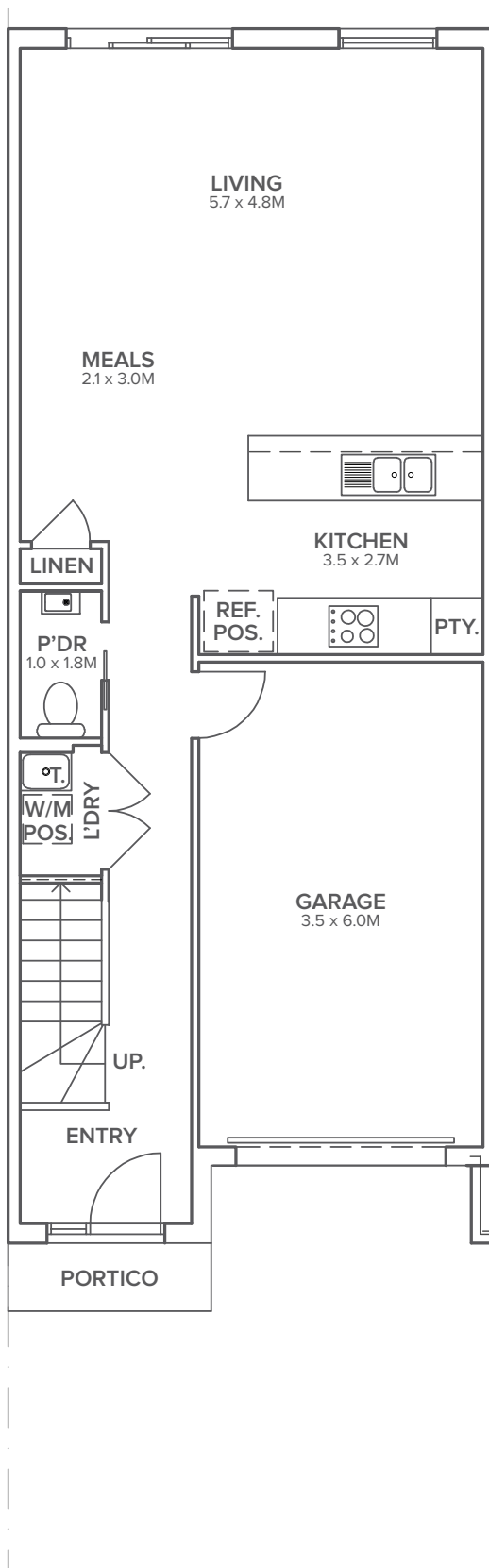
GROUND FLOOR
