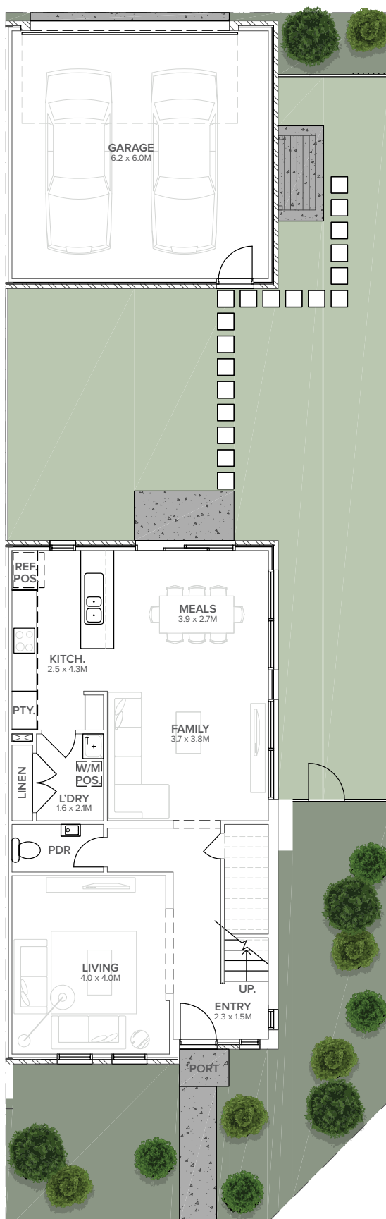
GROUND FLOOR
